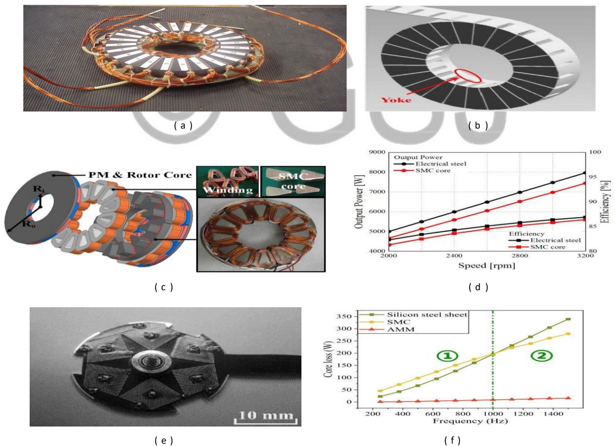
Fig. 4. AFPM stator examples: (a) Tapewound core with slots cut using EDM [29]; (b) Slotted stator using stamped lamination [31]; (c) AFPM using SMC core [34]; (d) Efficiency comparison between SMC and laminated stator [34]; (e) PCB windings [35]; (f) Core loss v/s frequency for laminated, SMC, and additively manufactured (AMM) stators [31];
