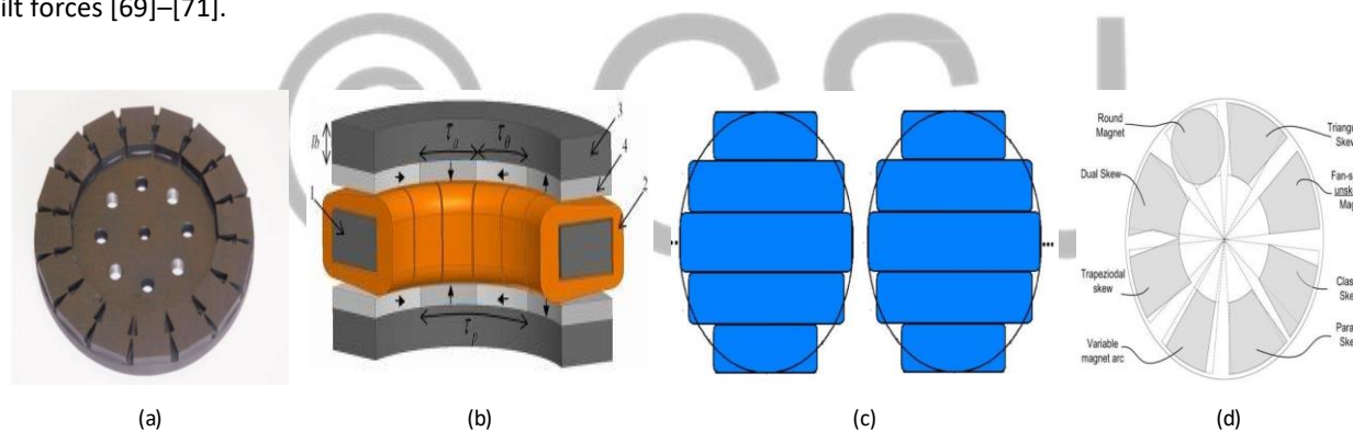
Fig. 5. (a) T-shaped PM with 14 cuboidal segments per pole [42]; (b) Torus machine with quasi-Halbach rotor [43]. The parts are 1 - stator core, 2 - toroidal winding, 3 - rotor core, and 4 - quasi Halbach array; (c) Circular pole shape using rectangular PM [44]; (d) Rotor skew techniques for AFPM [45]
