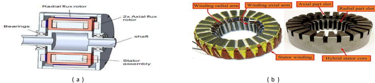
Fig. 6. Combined flux machines: (a) Cross-section of a combined flux PM vernier machine [78]; (b) Combined flux hysteresis machine stator [79]
