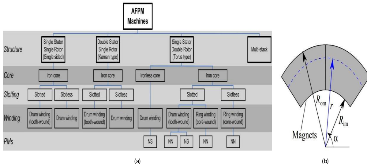
Fig. 1. (a) Classification of AFPM topologies [2]; (b) Main radial dimensions of an AFPM [11].
