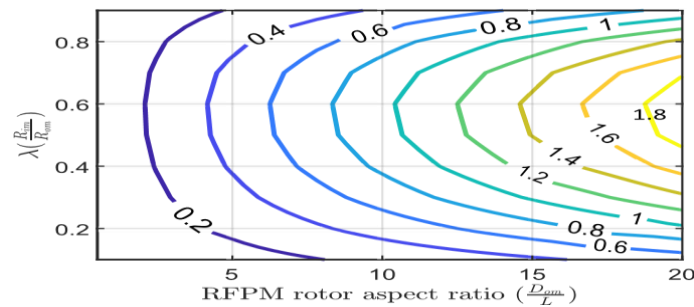
Fig. 2. Comparison of AFPM and RFPM torque capability
