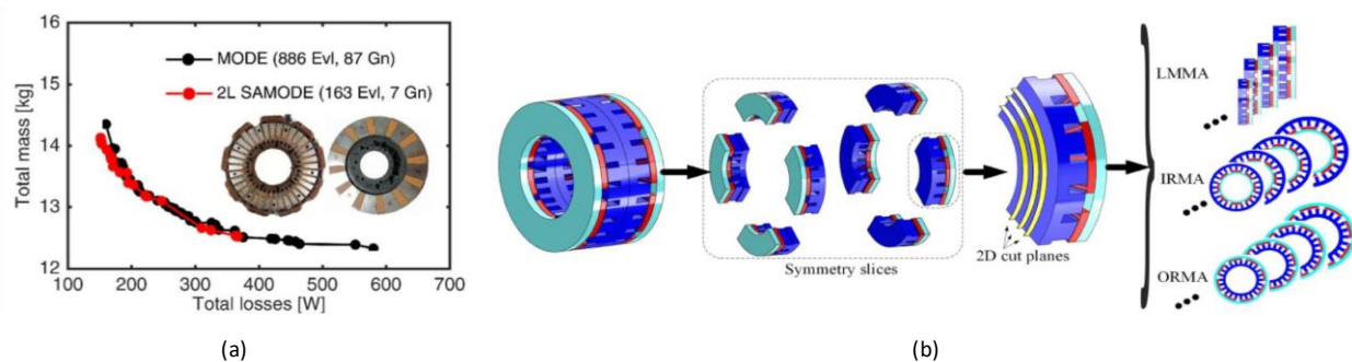
Fig. 3. (a) Comparison of Pareto fronts obtained using MODE and two level surrogate assisted MODE [7] for a commercial AFPM. Evi indicates the number of 3D FEA evaluations to reach the Pareto front.; (b) Schematic showing 2D modeling approaches for AFPM [22].
