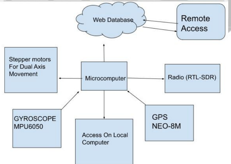
Fig: The Schematics of the electronics of the telescope.
