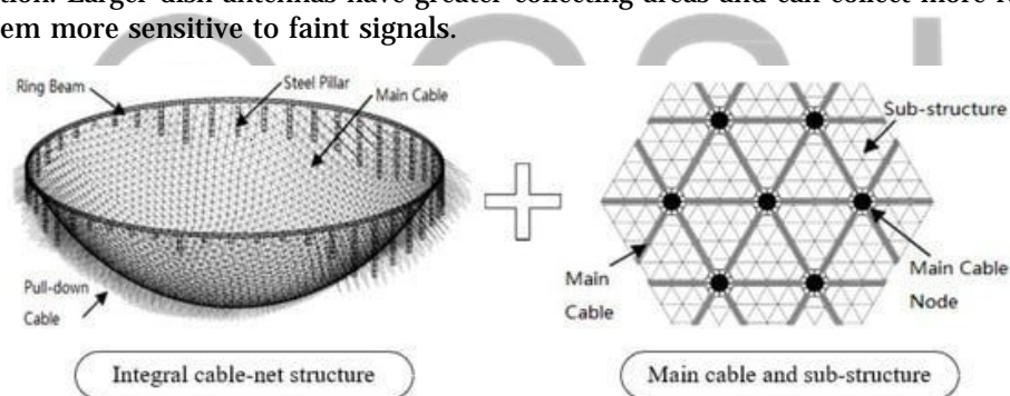
Fig:Structure of the antanae Dish [27].
