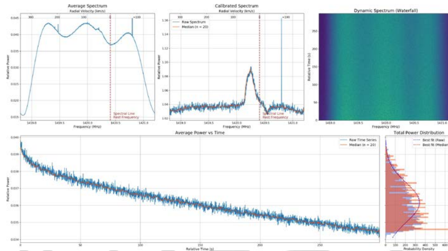
Fig: An Observed signals of HI Lines with the Virgo [24].
