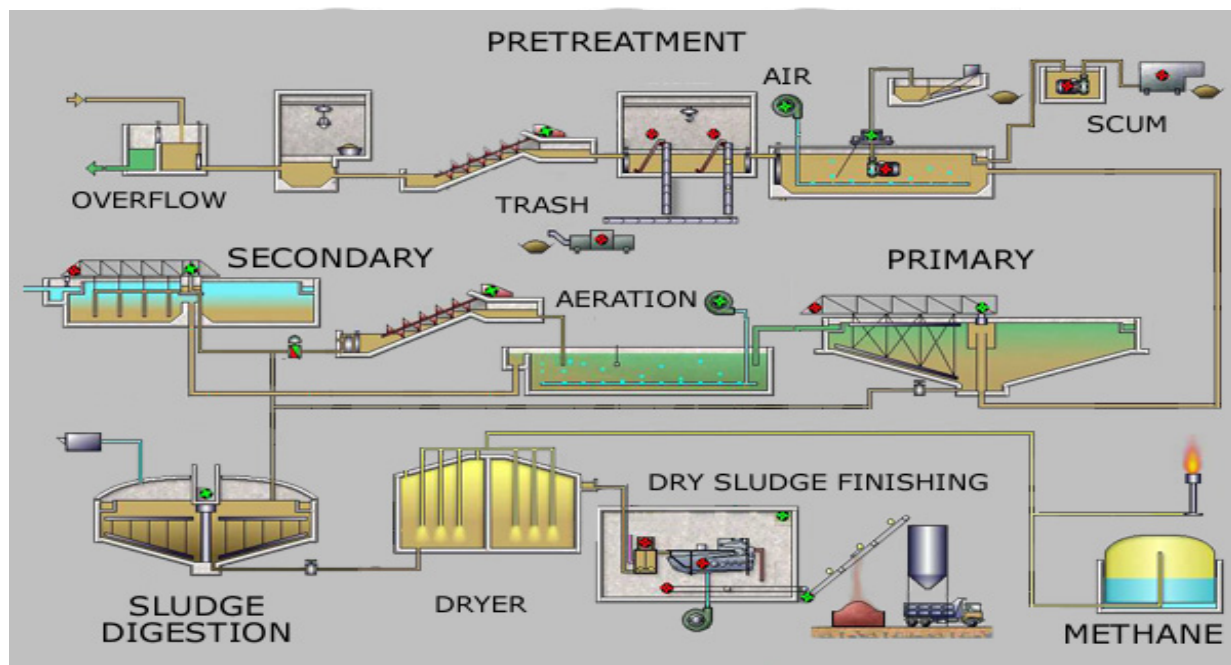
Figure 1: Simplified process flow diagram for a typical large-scale treatment [25].
