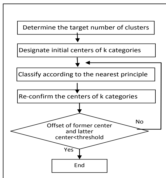
Figure 1. Algorithm of K-Means Clustering Analysis
