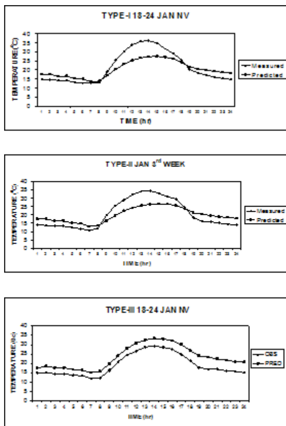
Fig. 8 Simulation results of greenhouse air temperature for month of January for different type of greenhouses (nv-natural ventilation; obs-observed; pred-predicted).
